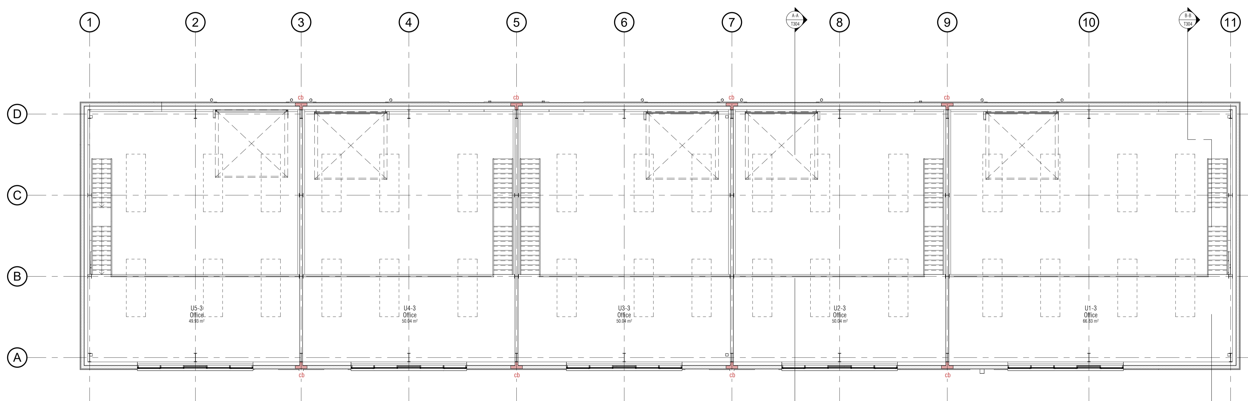
Lvl 00 - General Arrangement Plan 1:100
